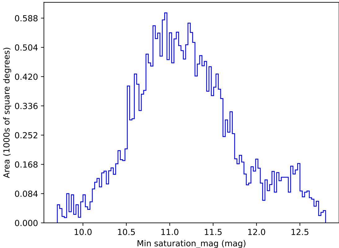
too_elab_r16_d2_gz_v3.4_10yrs All sky all bands: Min saturation_mag
