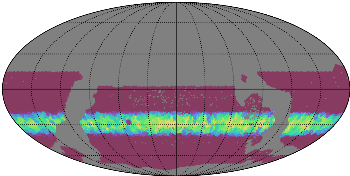
too_elab_r16_d2_gz_v3.4_10yrs WFD r band: Min normairmass
