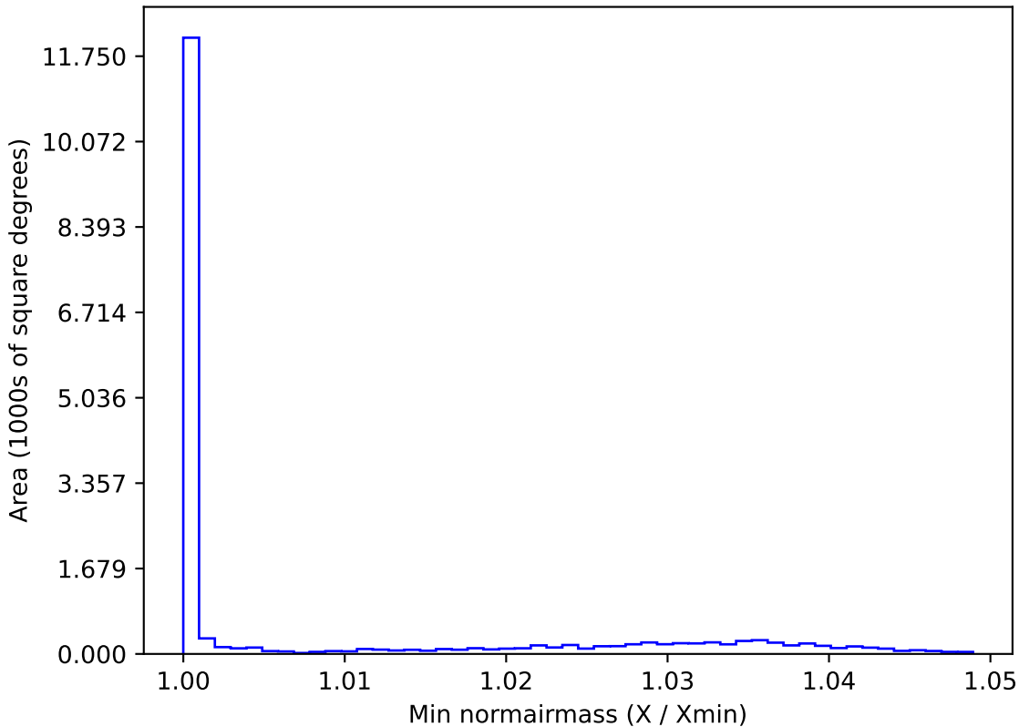
too_elab_r16_d2_gz_v3.4_10yrs WFD g band: Min normairmass
