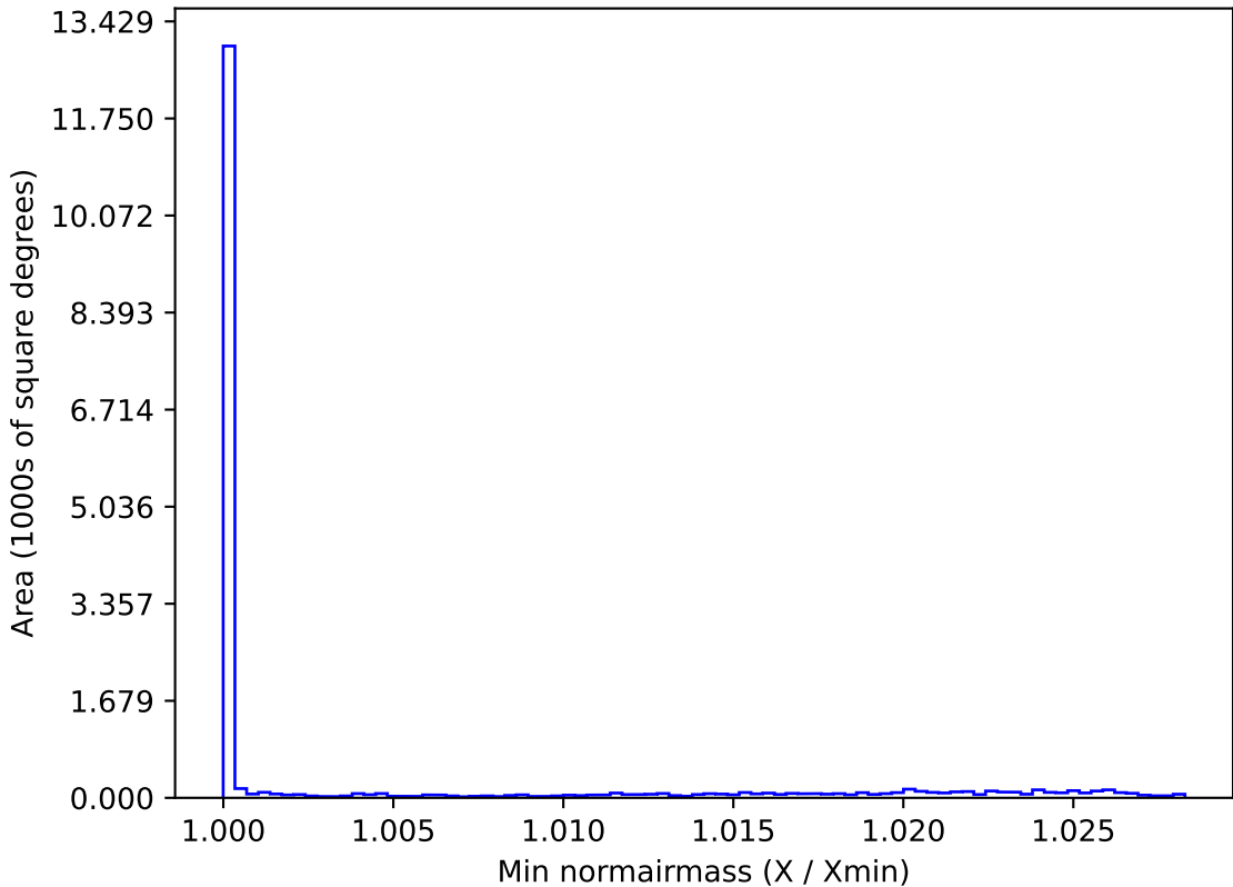
too_elab_r16_d2_gz_v3.4_10yrs WFD all bands: Min normairmass
