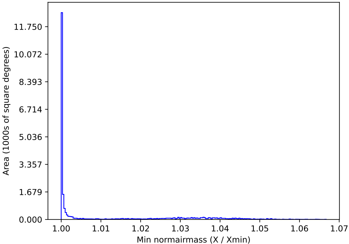
too_elab_r16_d2_gz_v3.4_10yrs All sky u band: Min normairmass
