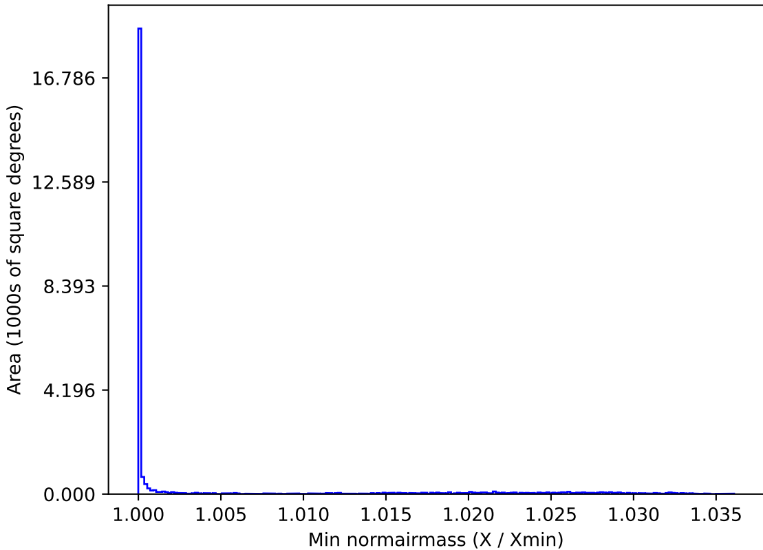
too_elab_r16_d2_gz_v3.4_10yrs All sky r band: Min normairmass
