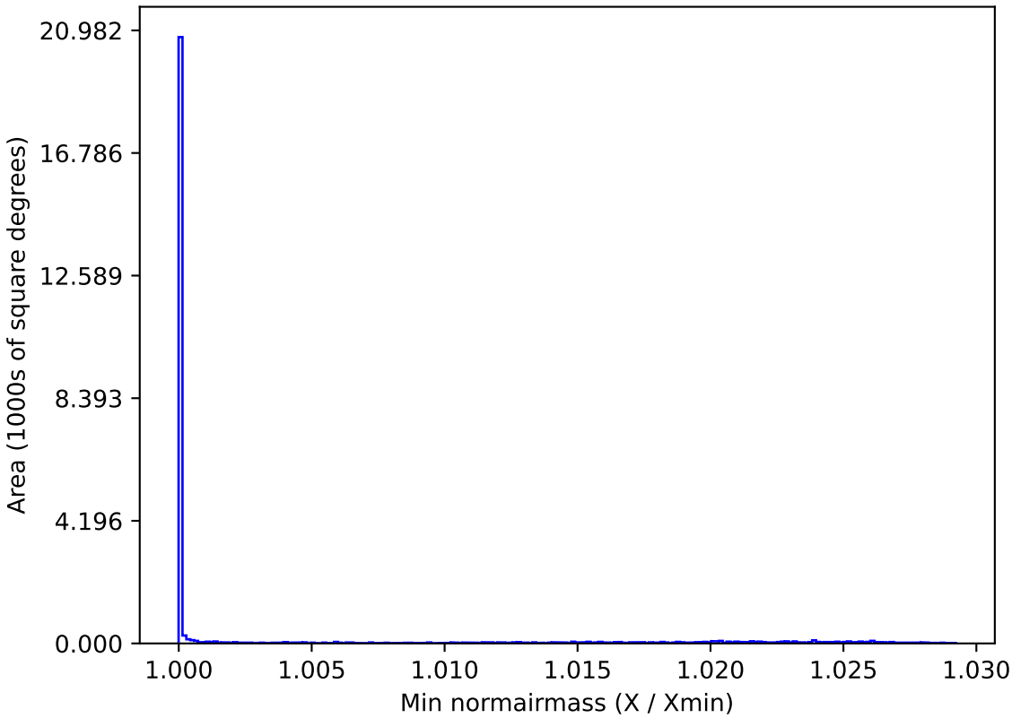
too_elab_r16_d2_gz_v3.4_10yrs All sky all bands: Min normairmass
