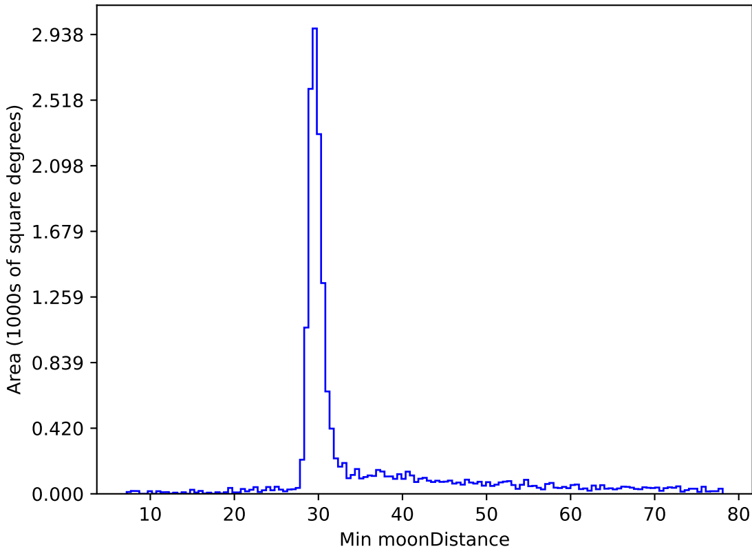
too_elab_r16_d2_gz_v3.4_10yrs WFD z band: Min moonDistance
