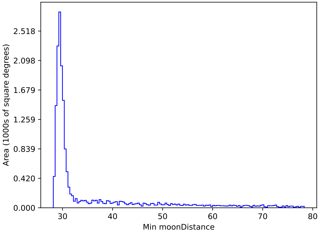
too_elab_r16_d2_gz_v3.4_10yrs WFD y band: Min moonDistance
