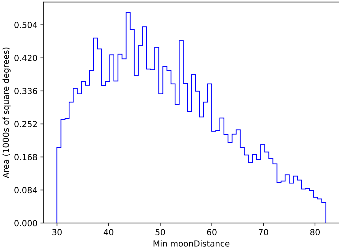
too_elab_r16_d2_gz_v3.4_10yrs WFD u band: Min moonDistance
