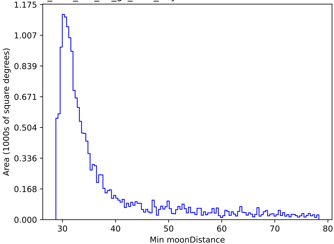
too_elab_r16_d2_gz_v3.4_10yrs WFD r band: Min moonDistance
