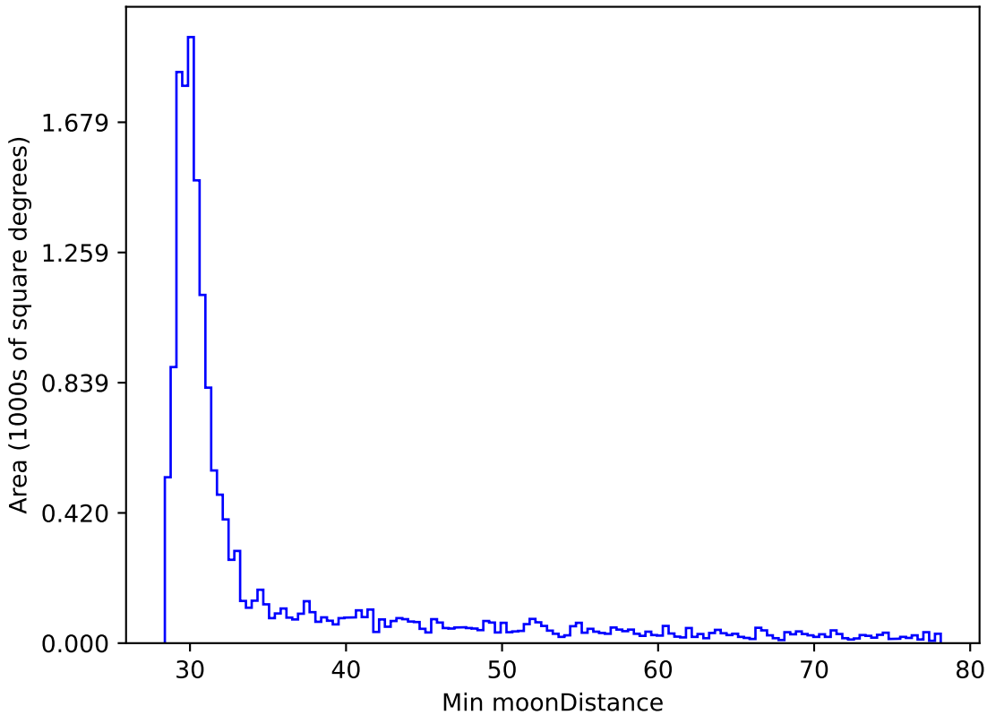
too_elab_r16_d2_gz_v3.4_10yrs WFD i band: Min moonDistance
