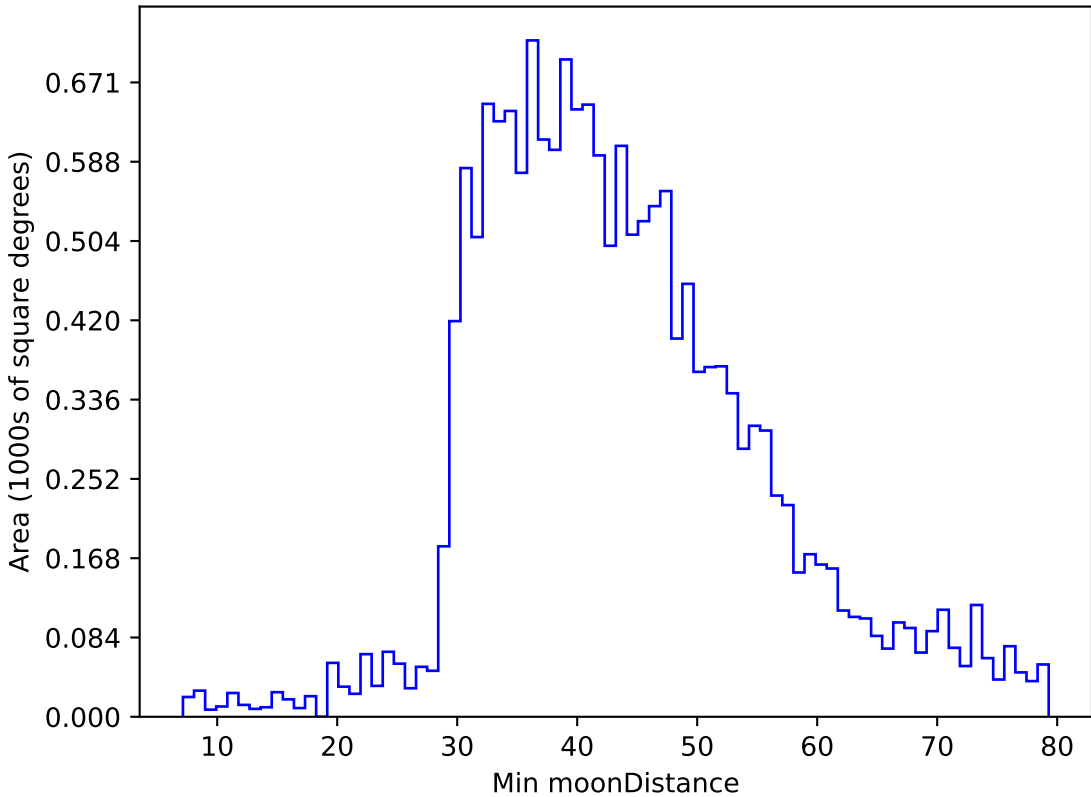
too_elab_r16_d2_gz_v3.4_10yrs WFD g band: Min moonDistance
