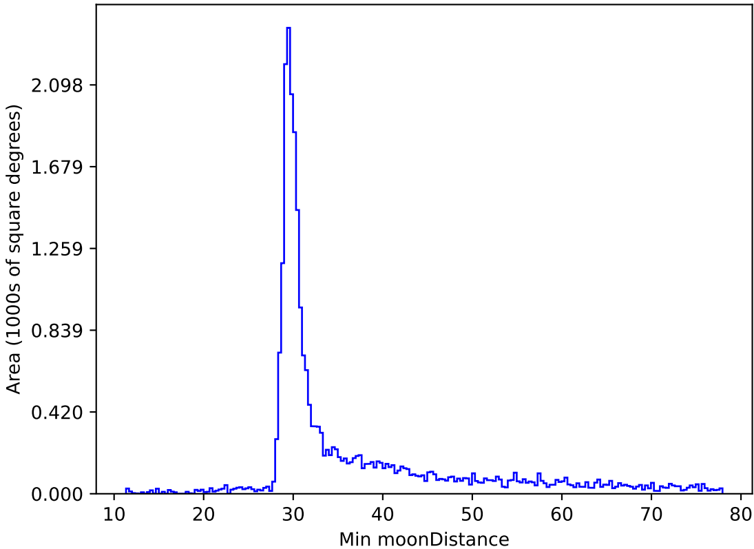
too_elab_r16_d2_gz_v3.4_10yrs All sky z band: Min moonDistance
