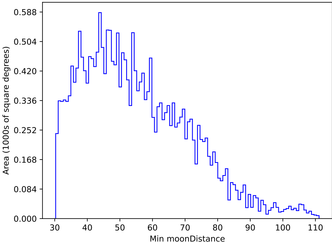
too_elab_r16_d2_gz_v3.4_10yrs All sky u band: Min moonDistance
