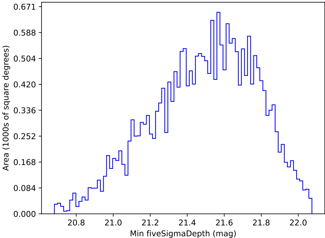
too_elab_r16_d2_gz_v3.4_10yrs Yr 1 y band: Min fiveSigmaDepth
