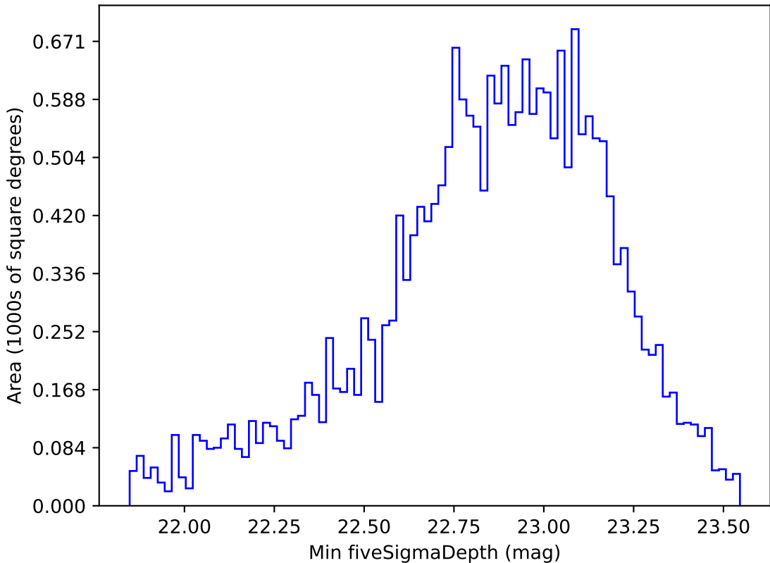
too_elab_r16_d2_gz_v3.4_10yrs Yr 1 u band: Min fiveSigmaDepth
