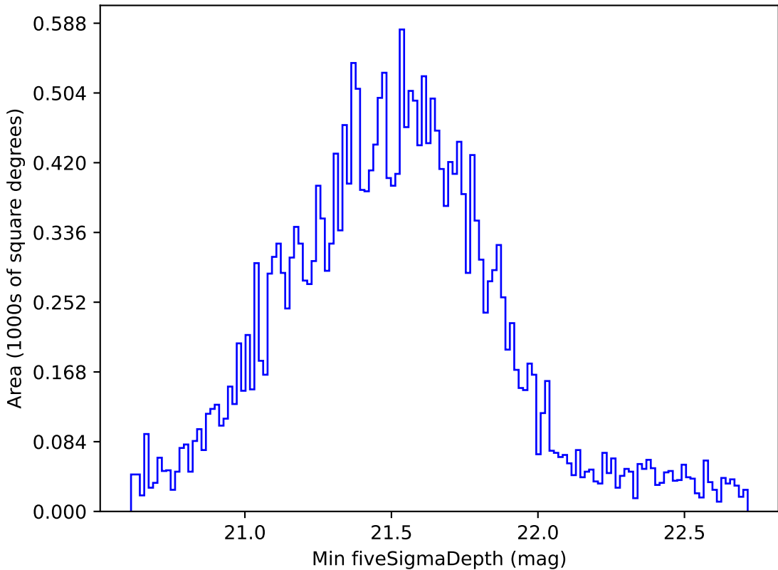
too_elab_r16_d2_gz_v3.4_10yrs Yr 1 all bands: Min fiveSigmaDepth
