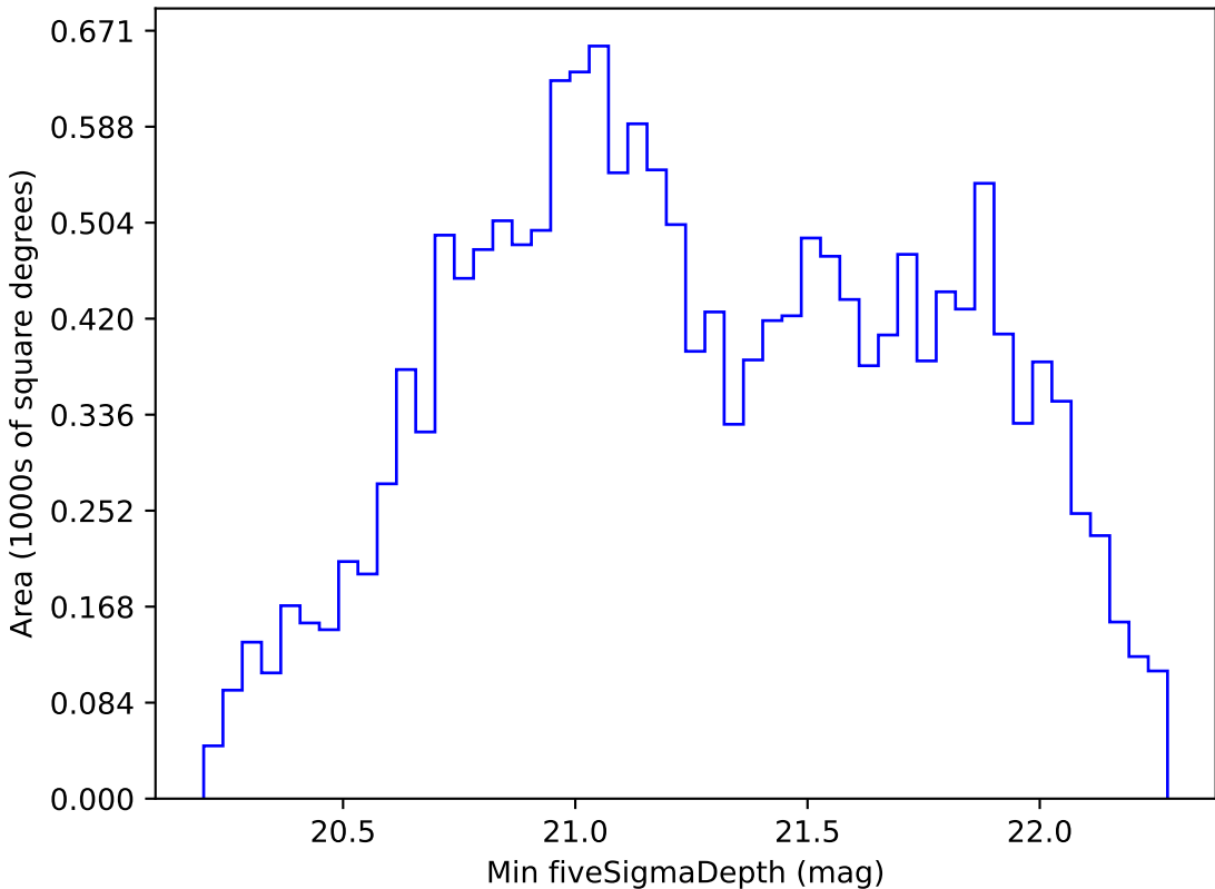
too_elab_r16_d2_gz_v3.4_10yrs WFD z band: Min fiveSigmaDepth
