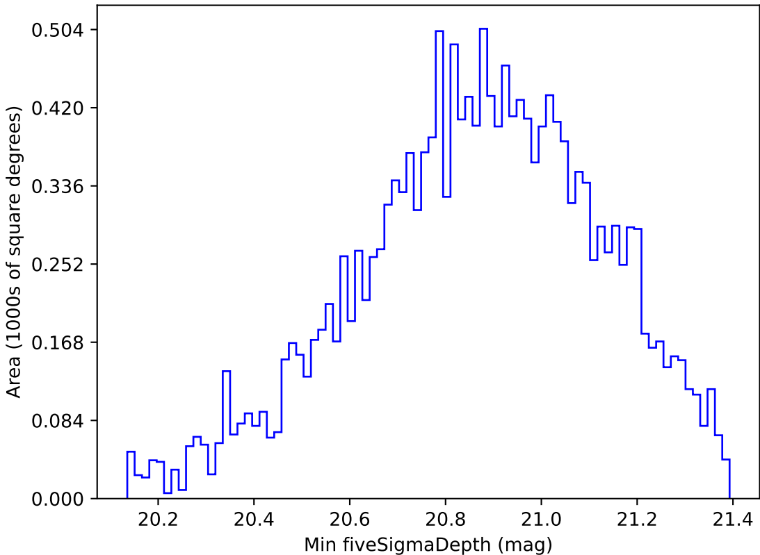
too_elab_r16_d2_gz_v3.4_10yrs WFD y band: Min fiveSigmaDepth
