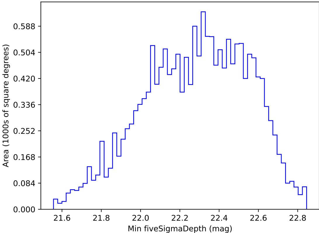
too_elab_r16_d2_gz_v3.4_10yrs WFD u band: Min fiveSigmaDepth
