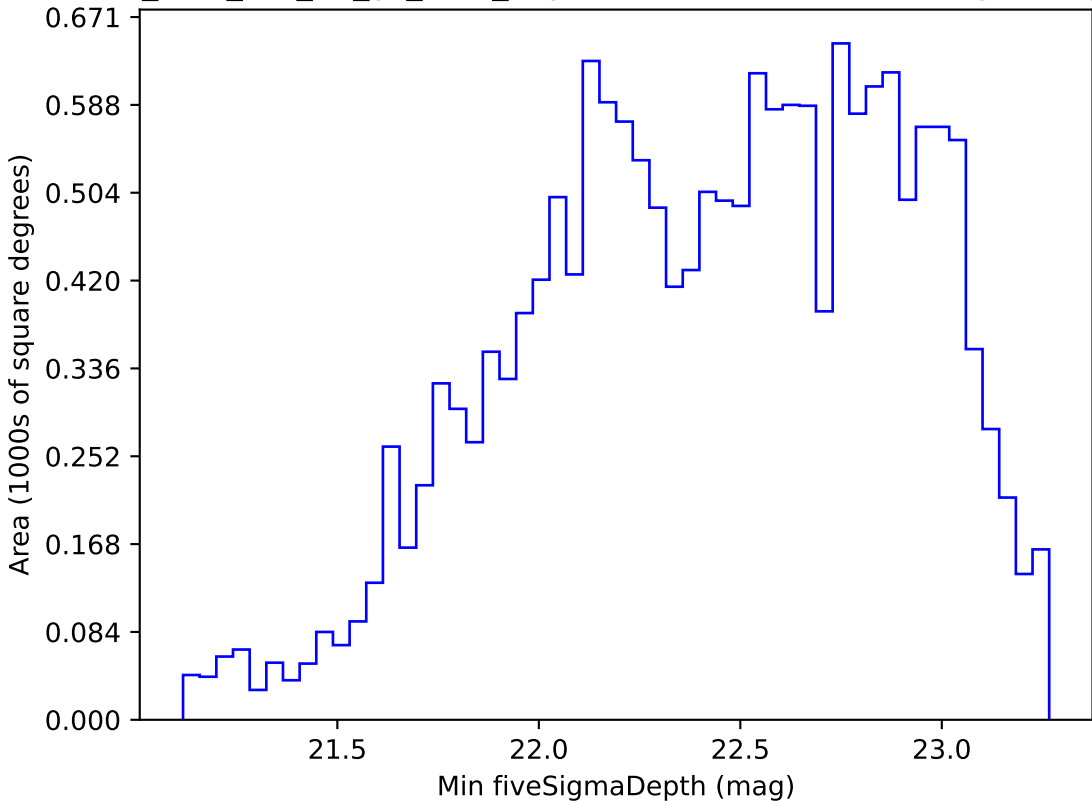
too_elab_r16_d2_gz_v3.4_10yrs WFD r band: Min fiveSigmaDepth
