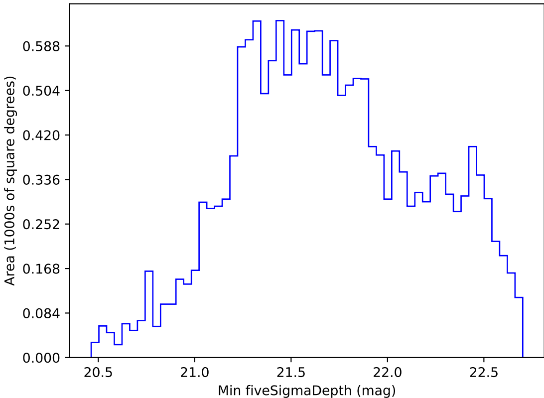
too_elab_r16_d2_gz_v3.4_10yrs WFD i band: Min fiveSigmaDepth
