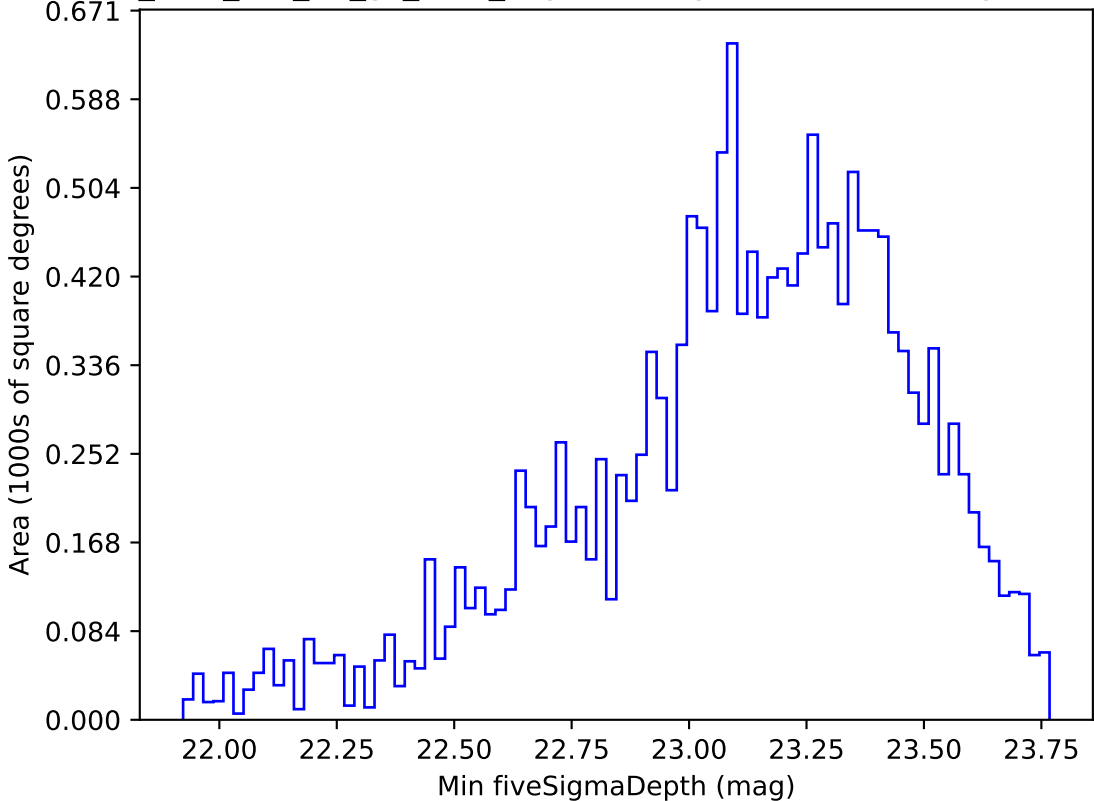
too_elab_r16_d2_gz_v3.4_10yrs WFD g band: Min fiveSigmaDepth
