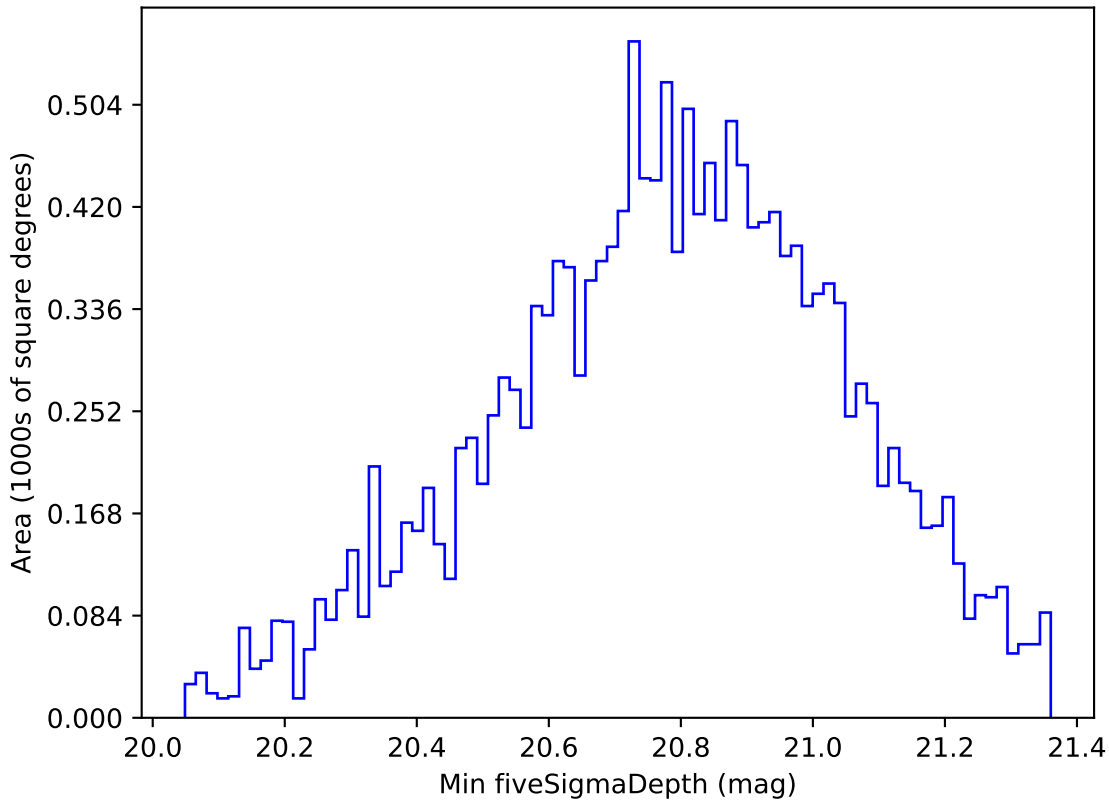
too_elab_r16_d2_gz_v3.4_10yrs WFD all bands: Min fiveSigmaDepth
