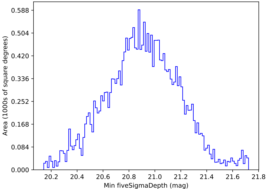
too_elab_r16_d2_gz_v3.4_10yrs All sky y band: Min fiveSigmaDepth
