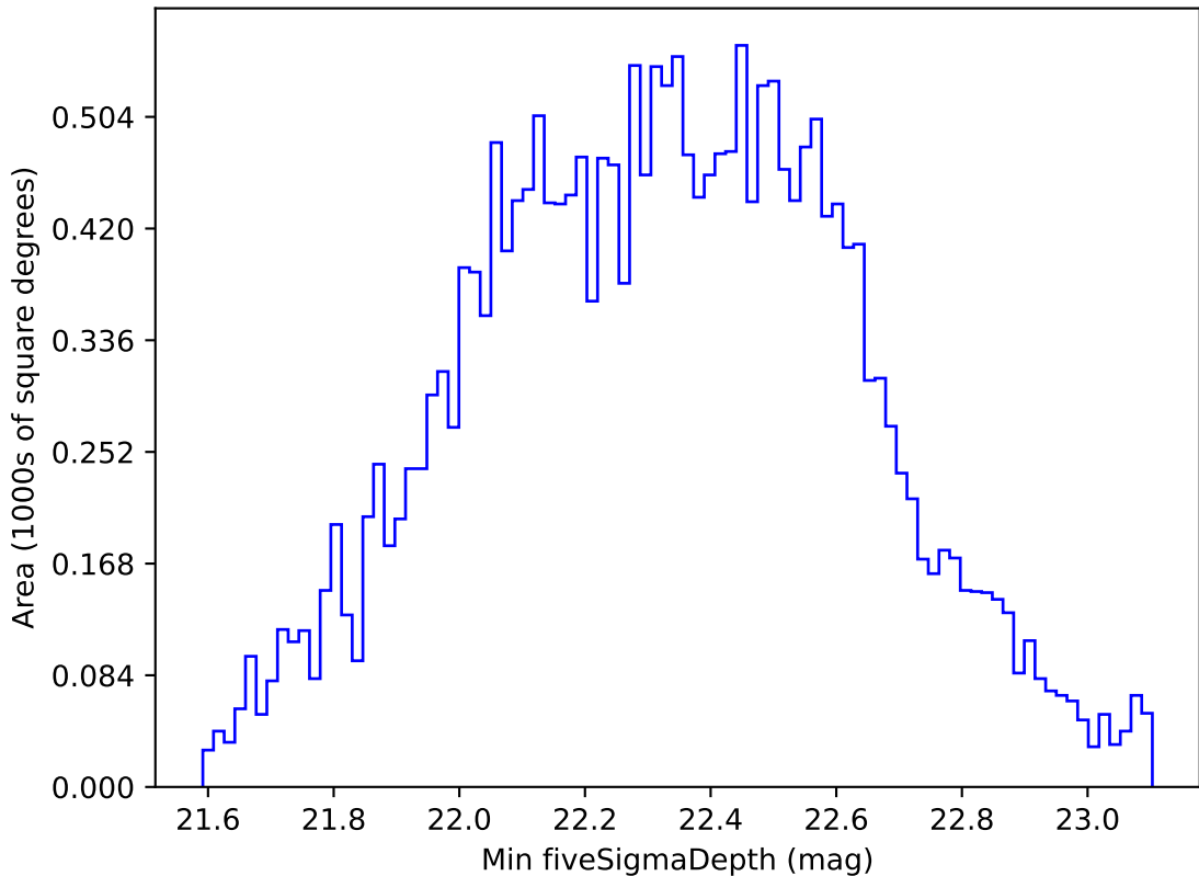
too_elab_r16_d2_gz_v3.4_10yrs All sky u band: Min fiveSigmaDepth
