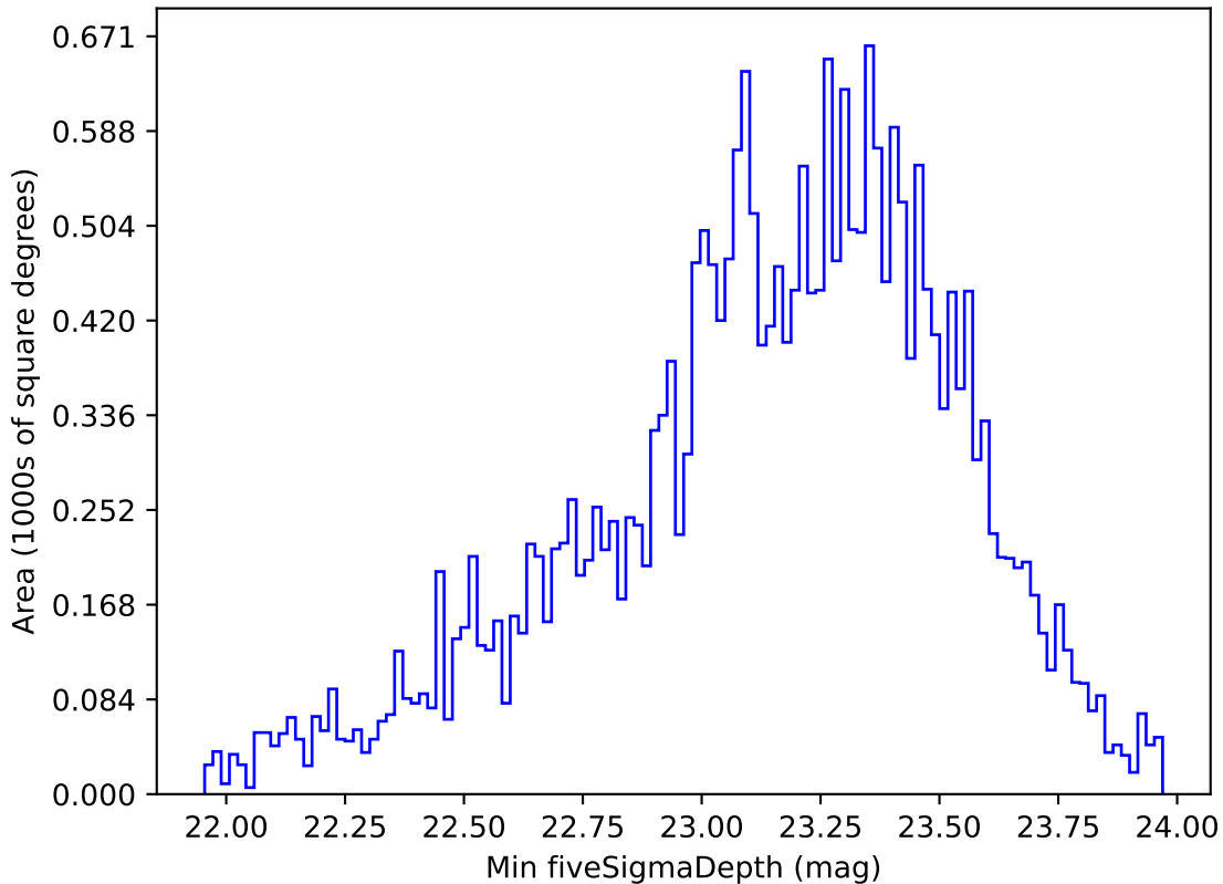
too_elab_r16_d2_gz_v3.4_10yrs All sky g band: Min fiveSigmaDepth
