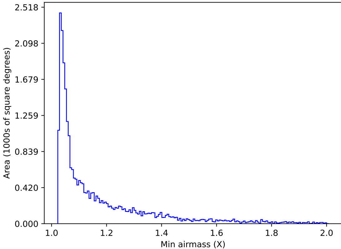
too_elab_r16_d2_gz_v3.4_10yrs Yr 1 z band: Min airmass
