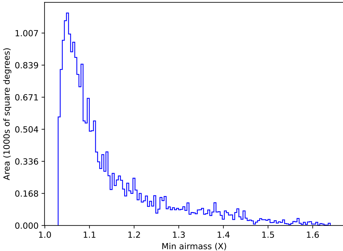
too_elab_r16_d2_gz_v3.4_10yrs Yr 1 u band: Min airmass
