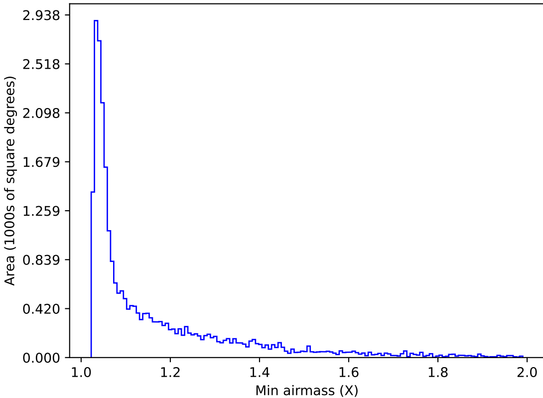
too_elab_r16_d2_gz_v3.4_10yrs Yr 1 r band: Min airmass
