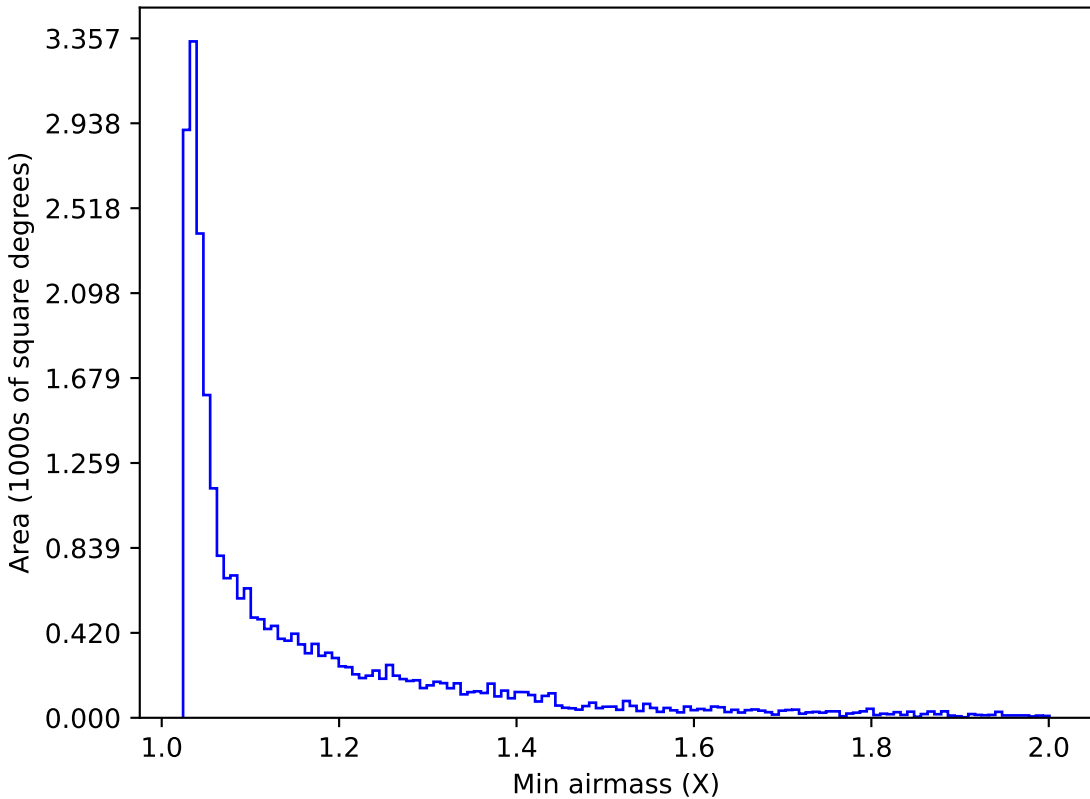
too_elab_r16_d2_gz_v3.4_10yrs Yr 1 i band: Min airmass
