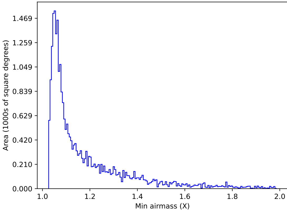
too_elab_r16_d2_gz_v3.4_10yrs Yr 1 g band: Min airmass
