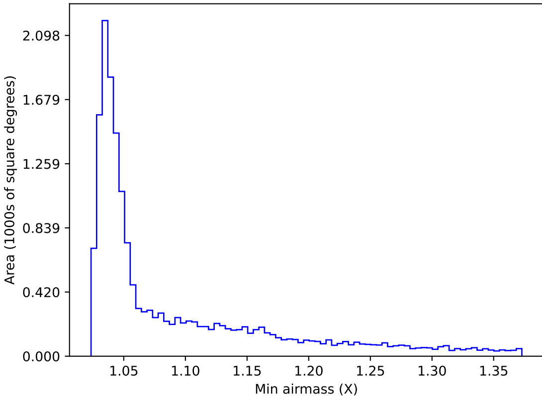
too_elab_r16_d2_gz_v3.4_10yrs WFD u band: Min airmass
