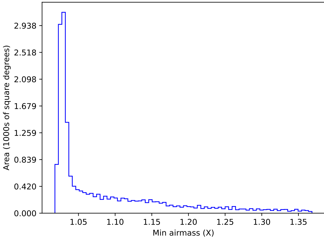
too_elab_r16_d2_gz_v3.4_10yrs WFD i band: Min airmass
