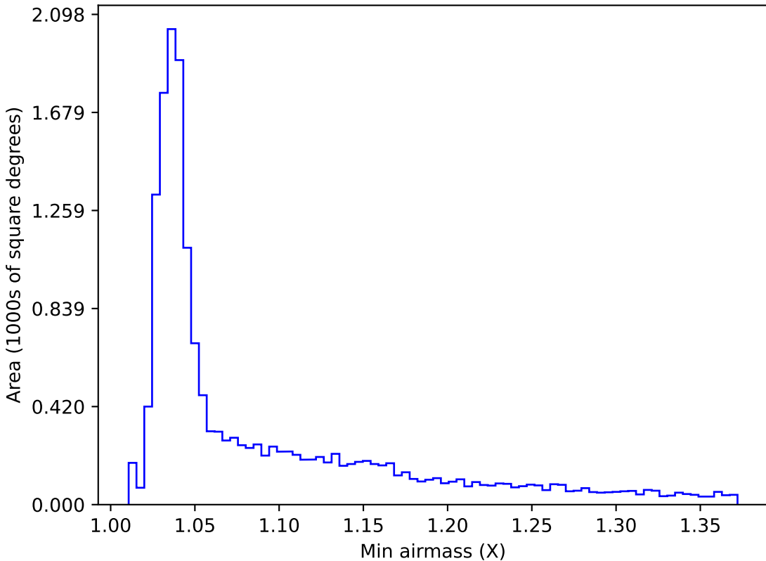
too_elab_r16_d2_gz_v3.4_10yrs WFD g band: Min airmass
