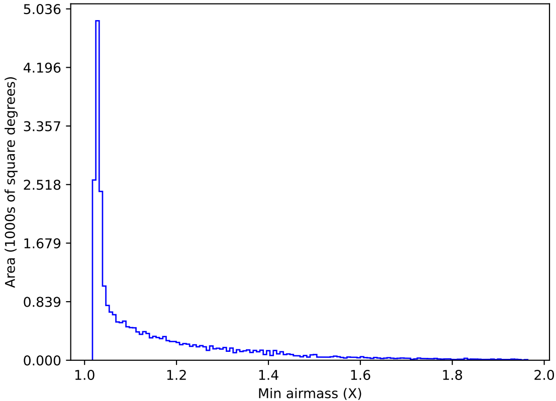
too_elab_r16_d2_gz_v3.4_10yrs All sky r band: Min airmass
