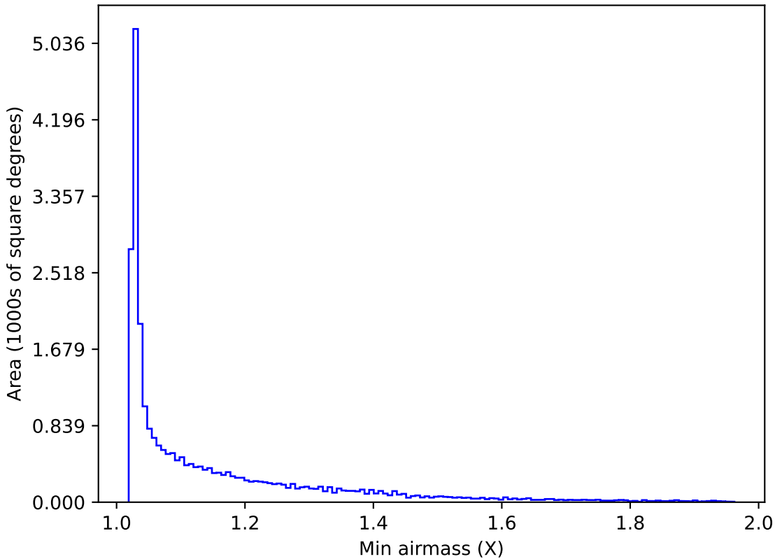
too_elab_r16_d2_gz_v3.4_10yrs All sky i band: Min airmass
