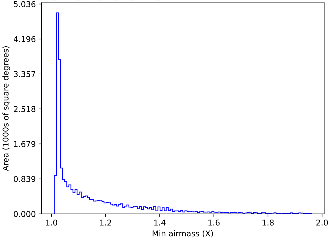
too_elab_r16_d2_gz_v3.4_10yrs All sky all bands: Min airmass
