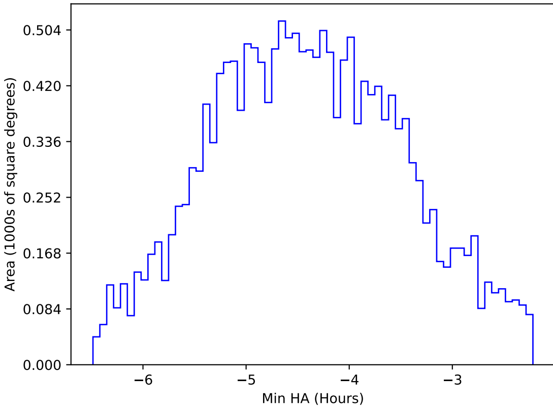
too_elab_r16_d2_gz_v3.4_10yrs WFD z band: Min HA
