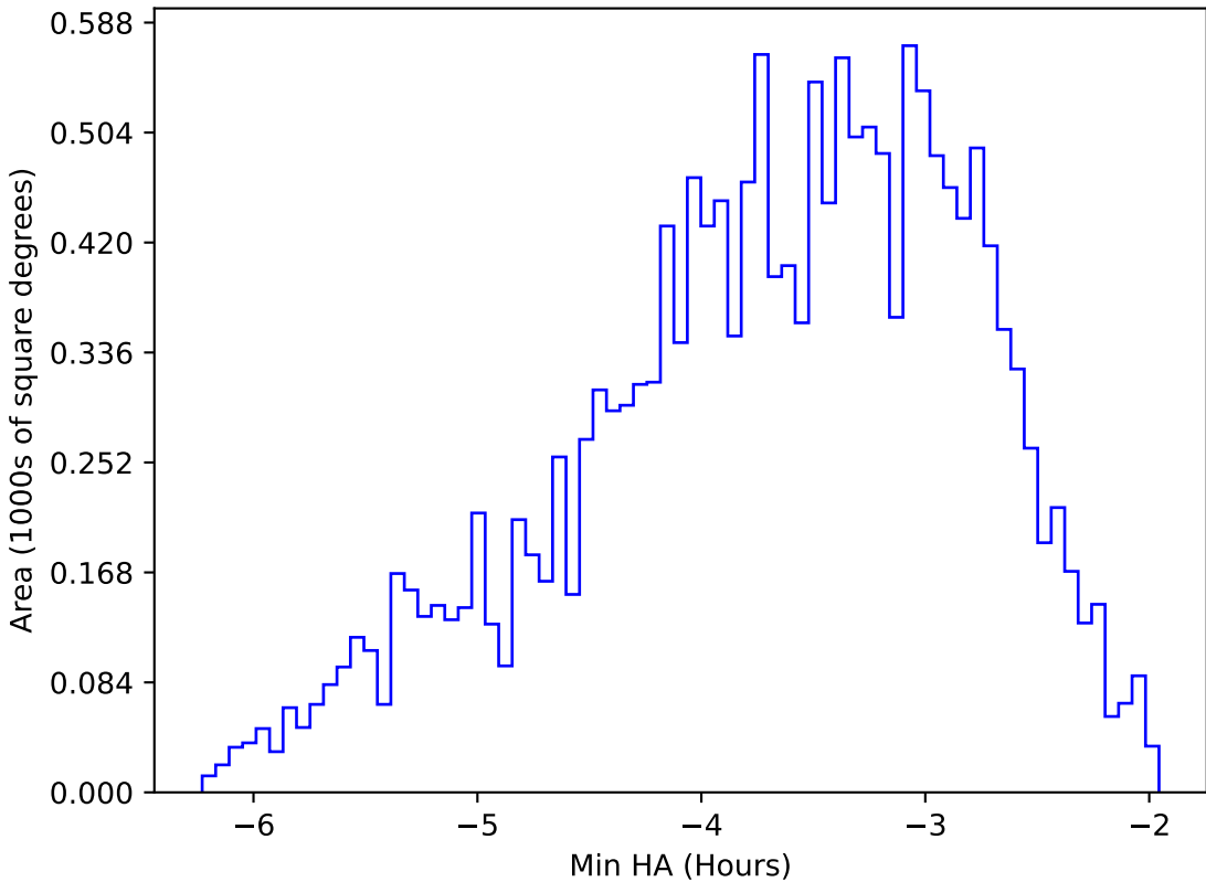
too_elab_r16_d2_gz_v3.4_10yrs WFD y band: Min HA
