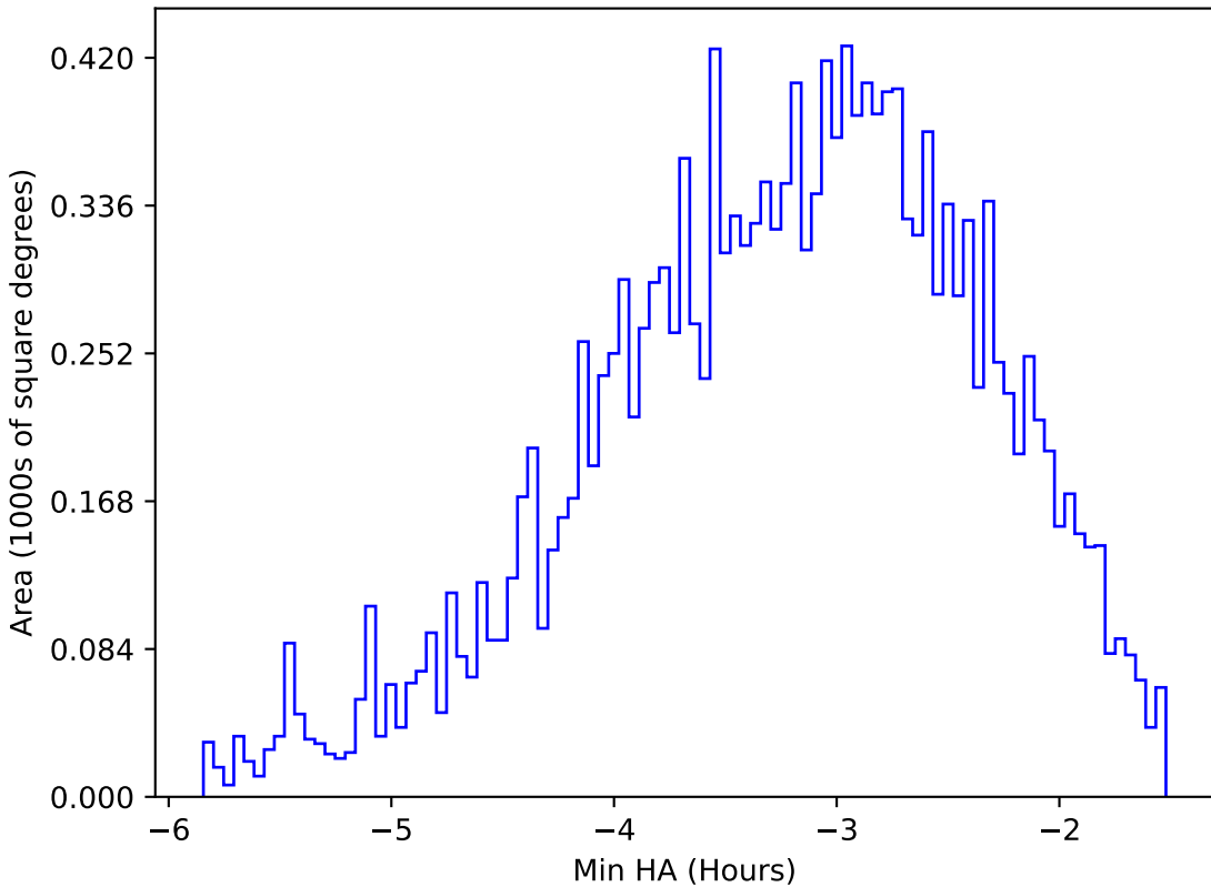
too_elab_r16_d2_gz_v3.4_10yrs WFD u band: Min HA
