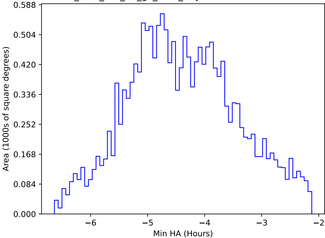
too_elab_r16_d2_gz_v3.4_10yrs WFD i band: Min HA
