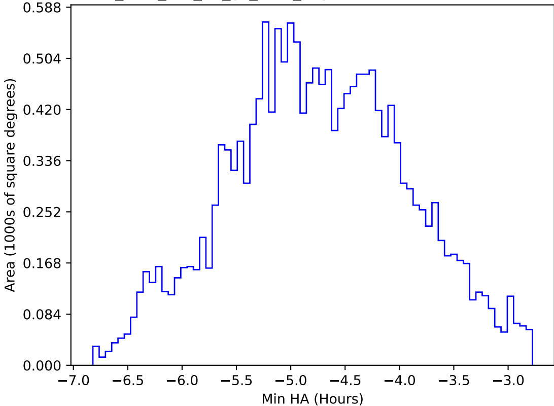
too_elab_r16_d2_gz_v3.4_10yrs WFD all bands: Min HA
