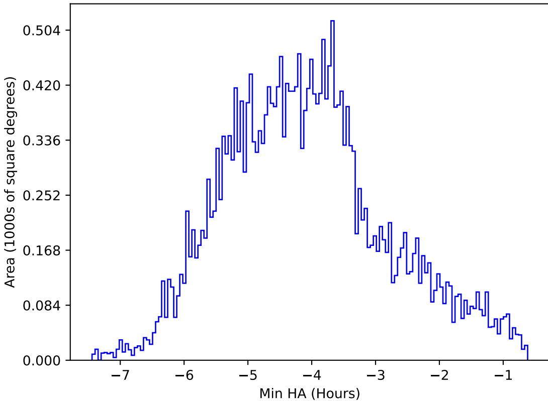
too_elab_r16_d2_gz_v3.4_10yrs All sky z band: Min HA
