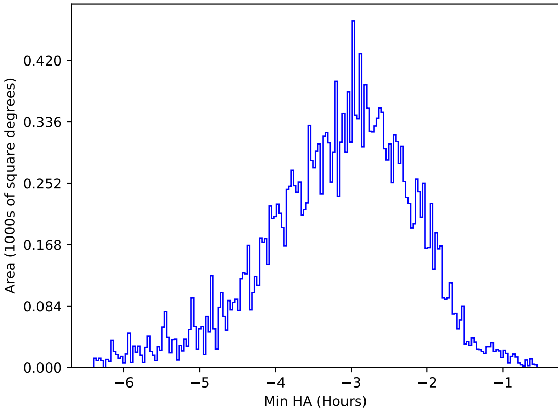
too_elab_r16_d2_gz_v3.4_10yrs All sky u band: Min HA
