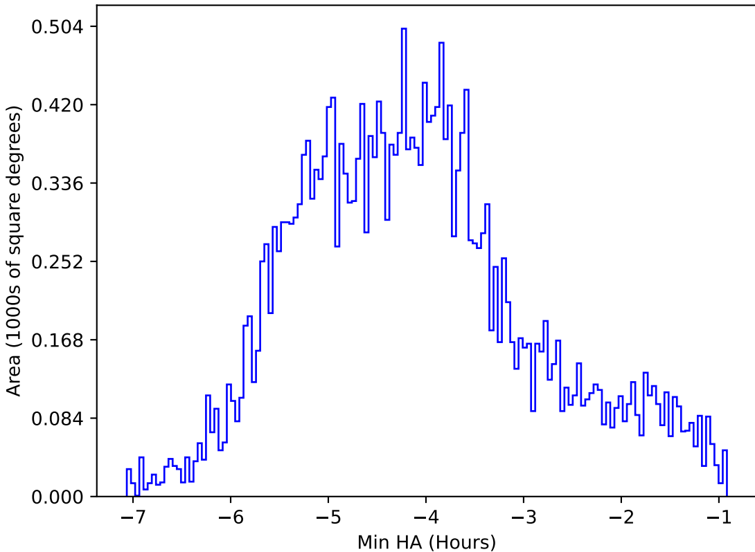
too_elab_r16_d2_gz_v3.4_10yrs All sky r band: Min HA
