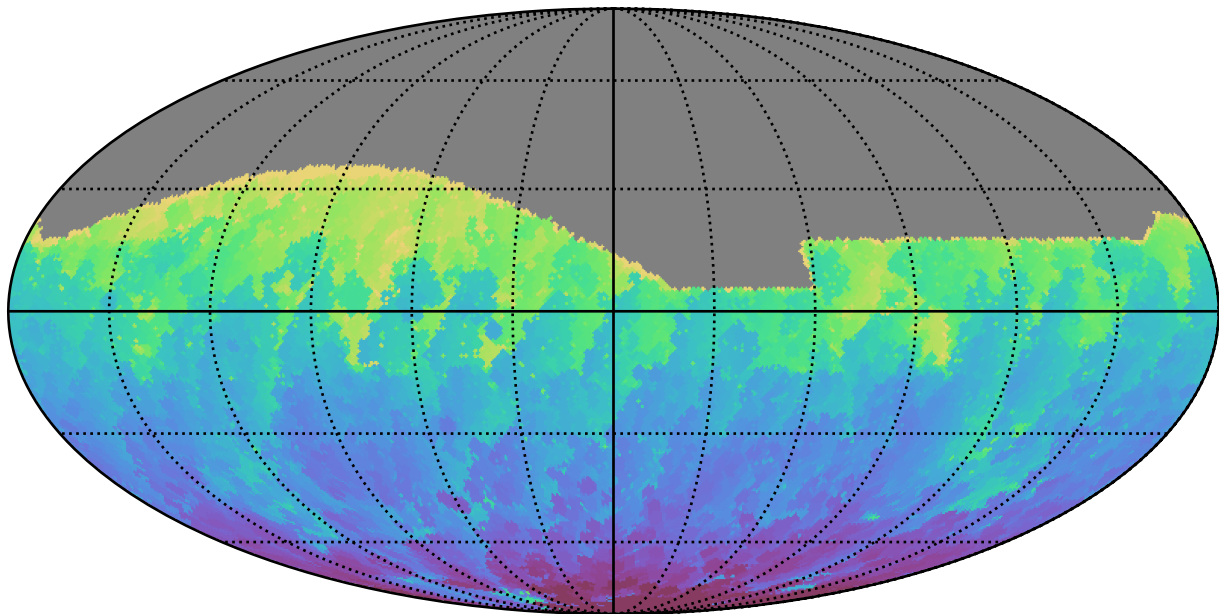
too_elab_r16_d2_gz_v3.4_10yrs All sky g band: Min HA
