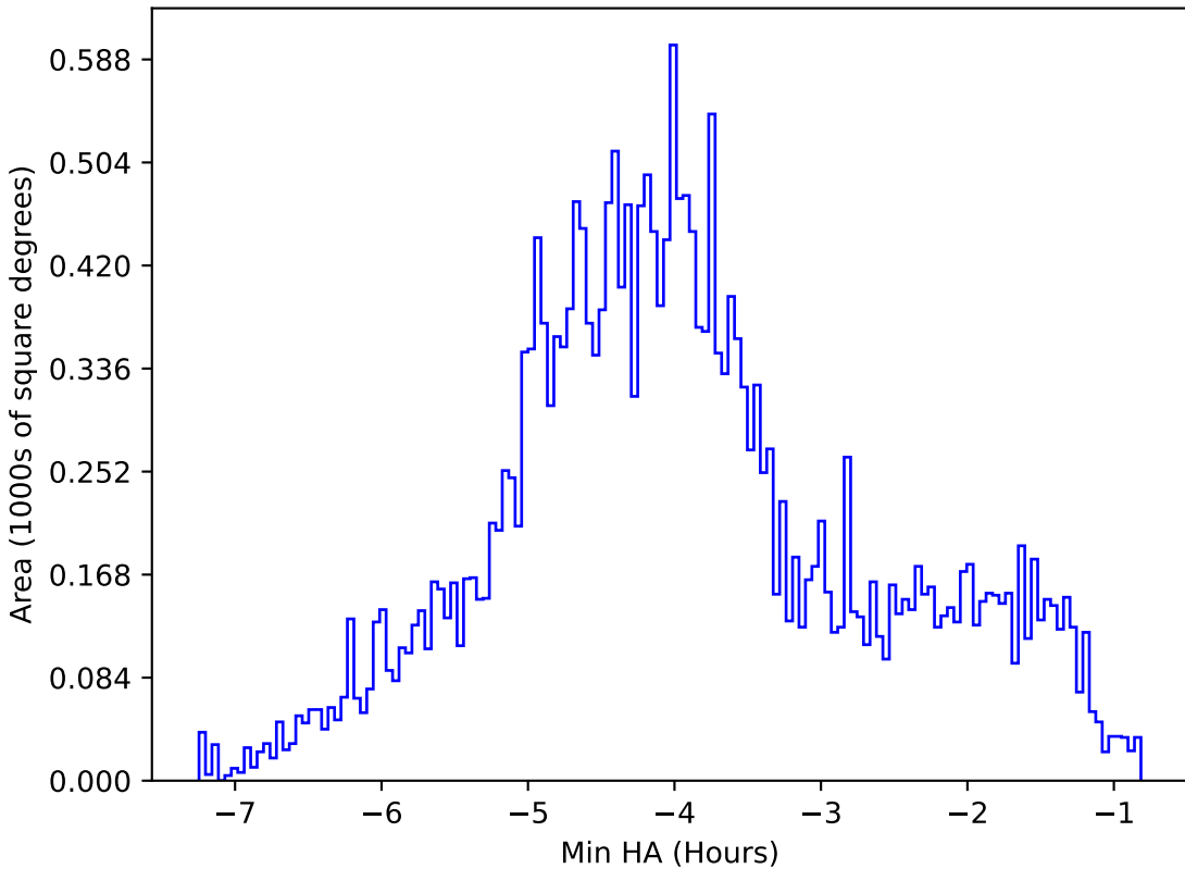
too_elab_r16_d2_gz_v3.4_10yrs All sky g band: Min HA
