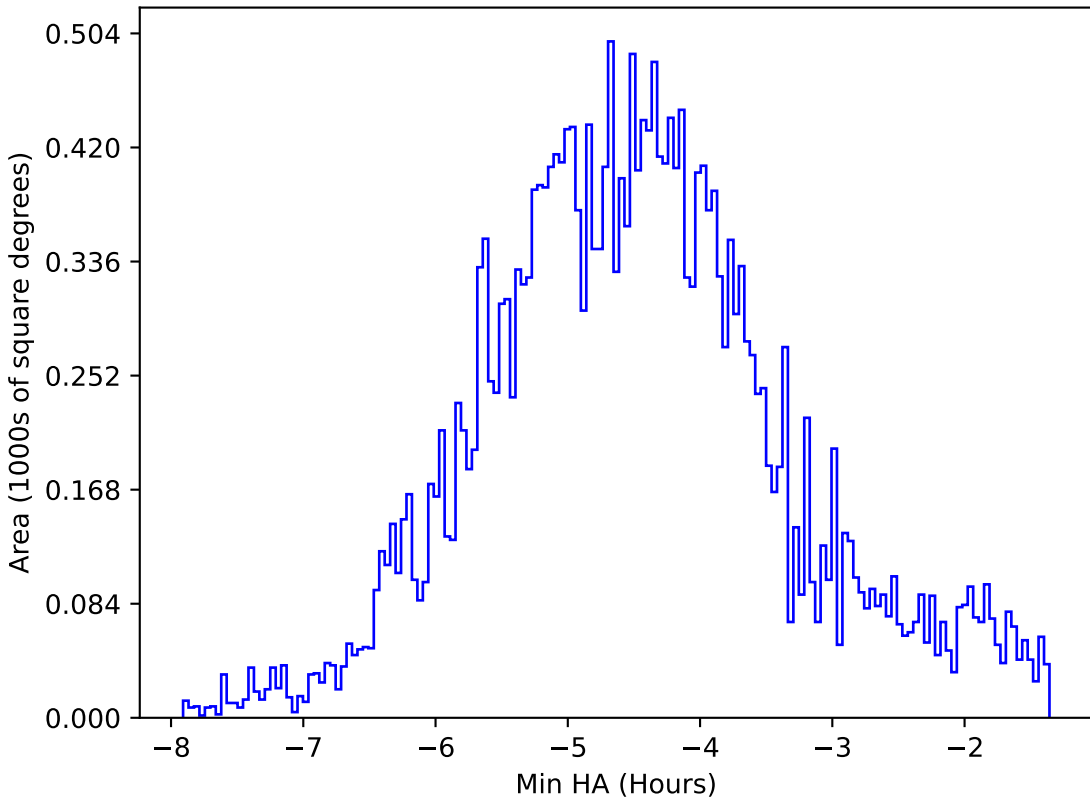
too_elab_r16_d2_gz_v3.4_10yrs All sky all bands: Min HA
